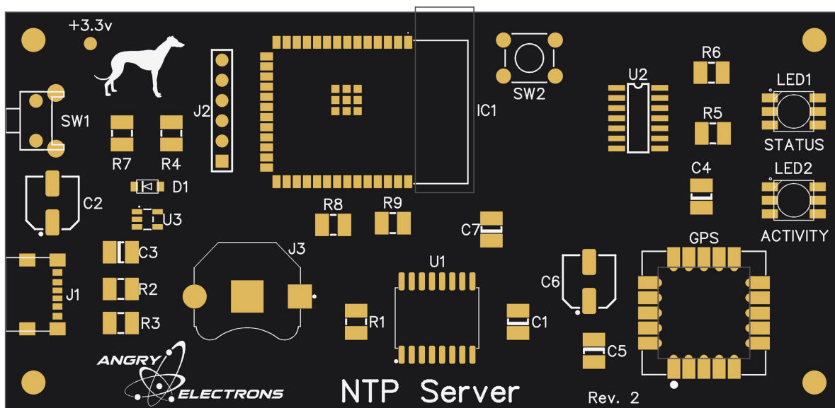
Figure 1 — Top-side component placement (Rev. 2 silkscreen). IC1 is the ESP32-S3 module; the GPS receiver is at the lower right.
